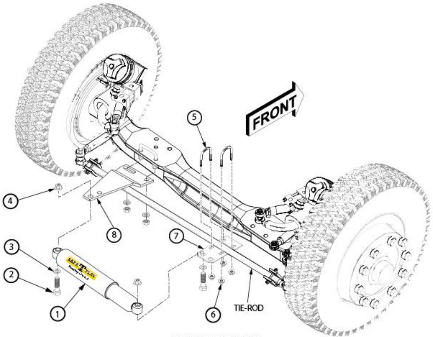
FRONT AXLE ASSEMBLY (Front axle assembly shown is typical and may not be an exact representation of your vehicle.)
